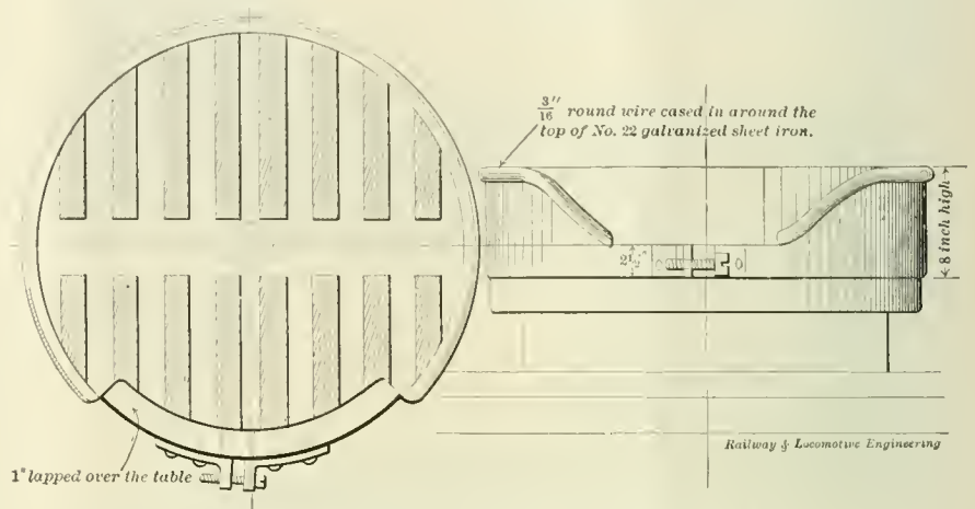
SHIELD FOR SLOTTOR TO PREVENT CHIPS FLYING.
